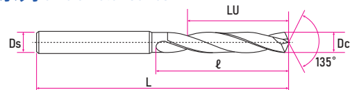
最大推荐钻深 Maximum recommended drilling depth LU=l-1.5D
